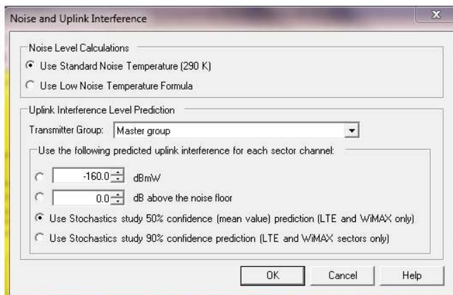
Dialog box for global uplink noise and interference prediction setup
