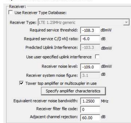
LTE sector receiver parameters showing predicted uplink noise and interference levels:
